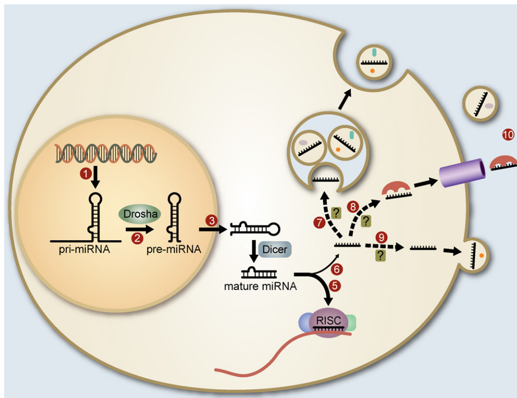
Fig. 1. The biogenesis of miRNAs. miRNA biogenesis begins with transcription of pri-miRNA transcripts by RNA polymerase II or III (1). In the nucleus, pri-miRNAs are processed by Droscha to produce pre-miRNA hairpins (2), which are then exported into the cytosol (3). Here, pre-miRNA hairpins are processed into 19–24 nucleotide mature miRNA duplexes by Dicer (4). One strand of the mature miRNA duplex is incorporated into the RISC complex where it can regulate expression of target mRNAs (5). The other strand may either be degraded, or possibly prepared for export from the cell (6). Some miRNAs have been found packaged in exosomes derived from multivesicular bodies (7). Others may be exported in the presence of RNA-binding proteins (8). Still others might be exported microvesicles shed during membrane blebbing (9). Once in the extracellular space, these miRNAs could be taken up by other cells, degraded by RNases, or excreted (10).
