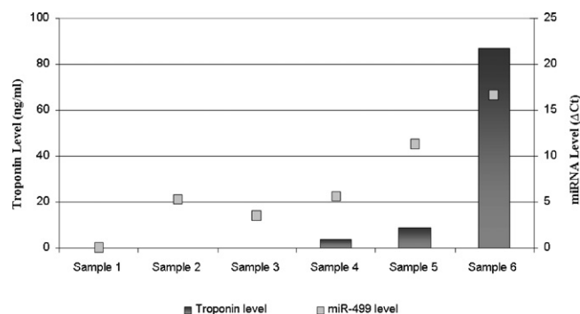
Fig. 2. Plasma miR-499 levels in patients with myocardial infarction. The concentration of plasma troponin (bars) and miR-499 (gray squares) was determined from 6 individuals (X-axis) whom may suffer myocardial infarction. The concentration of troponin was displayed as ng/ml and the level of miR-499 was presented in \Delta Ct value (40-Ct).
