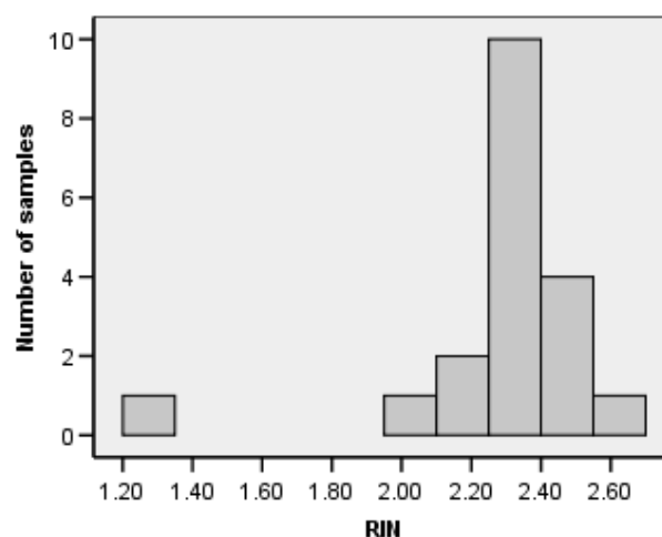
Fig. 7. A histogram of the RIN index in the examined samples.
