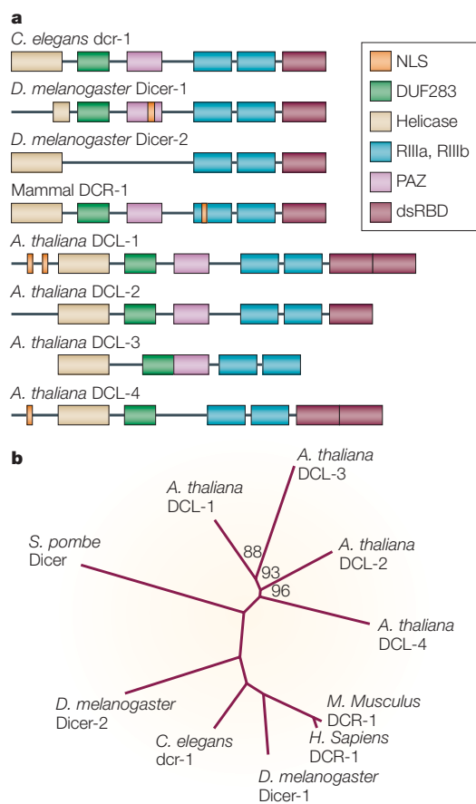
Figure 3 | The structure and function of the Dicer family. a | The domain structure of Dicer homologues in worms, flies, mammals and plants. The Dicer homologues that function in the microRNA (miRNA) maturation pathway have the PAZ (Piwi–Argonaute–Zwille) domain. b | The phylogenetic tree of the Dicer protein family. Multiple sequence alignment was done using ClustalW (version 1.80). PHYLIP95 (see online links box) was used to do BOOTSTRAP SAMPLING, protein-distance calculation (using Dayhoff PAM distance) and tree construction. Bootstrap percentages are indicated at each fork when the percentage is below 100. A. thaliana , Arabidopsis thaliana ; C. elegans , Caenorhabditis elegans ; D. melanogaster , Drosophila melanogaster ; H. sapiens , Homo sapiens ; M. musculus , Mus musculus ; RBD, RNA binding domain; S. pombe , Schizosaccharomyces pombe .
